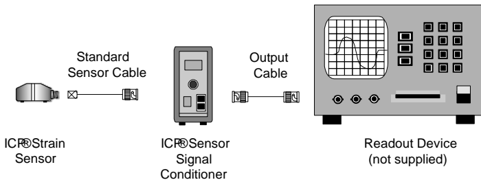
Figure 1.2 Typical ICP® Sensor System
