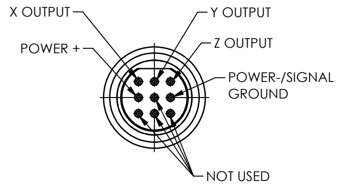
PIN OUT
